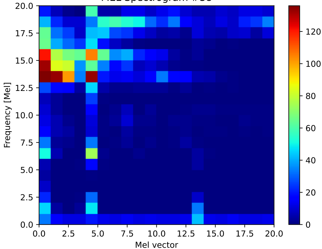
MEL Spectrogram #38
